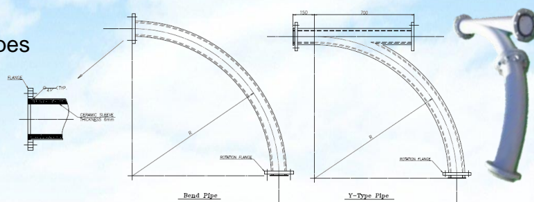
Elbow Pipe with Ceramic Liner
